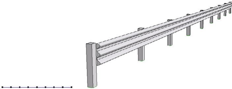
A polyline with nine nodes generates a guardrail with nine uprights
